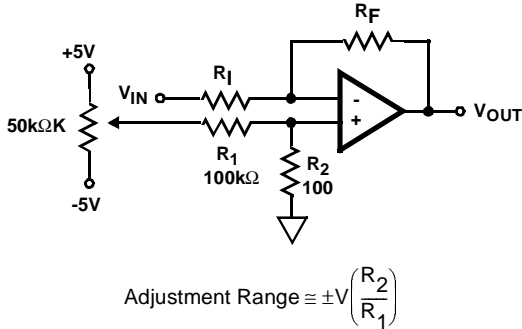
FIGURE 28. INVERTING GAIN
